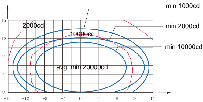
APPS-12-LED (White), ICAO Figure A2-1 (Vertical main beam coverage 0^\circ-11^\circ )
