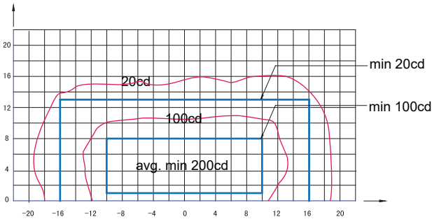
SBLM-08 (Red), ICAO Figure A2-12
